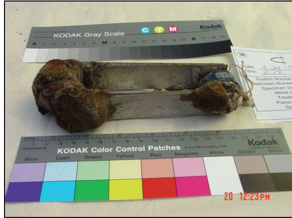
Above Left: U-bend stressed corrosion samples upon recovery (April 2004).
